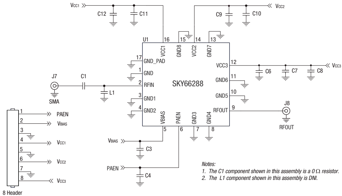
Figure 27. SKY66288-11 Evaluation Board Schematic
